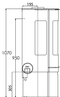
WESTFIRE.UNIQ.36 WESTFIRE.UNIQ.37 PEDESTAL 2 / WEIGHT: 95 KG
