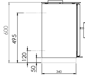
WESTFIRE.UNIQ.23 / PEDESTAL 5 FLAT / CURVED DOOR WEIGHT: 92 KG
