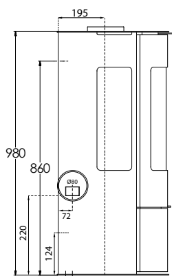
WESTFIRE.UNIQ.36 WESTFIRE.UNIQ.37 WEIGHT: 90 KG
