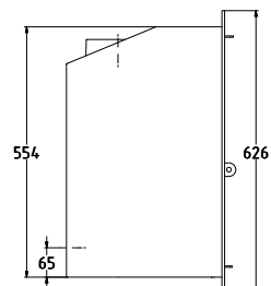
WESTFIRE.UNIQ.35 / INSERT 4-SIDED FRAME WEIGHT: 75 KG
