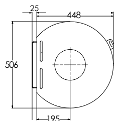
WESTFIRE.UNIQ.36 WESTFIRE.UNIQ.37 LEGS / WEIGHT: 85 KG
