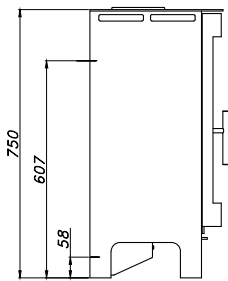
WESTFIRE.UNIQ.17 WEIGHT: 84 KG
