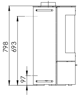
WESTFIRE.UNIQ.21 WEIGHT: 81 KG
