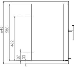
WESTFIRE.UNIQ.23 INSERT 4-SIDED FRAME FLAT / CURVED DOOR WEIGHT: 92 KG
