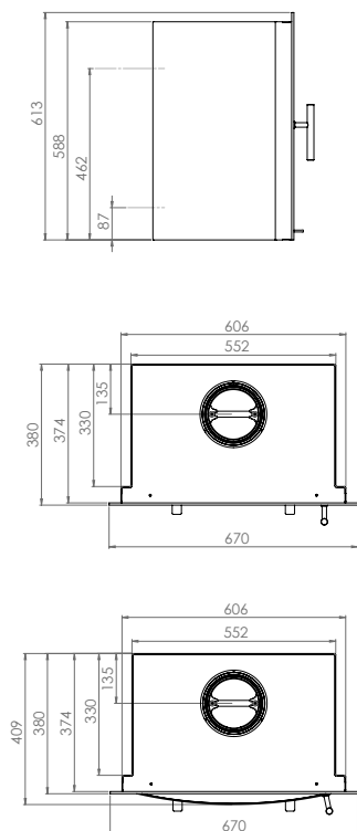
WESTFIRE.UNIQ.23 INSERT 3-SIDED FRAME FLAT / CURVED DOOR WEIGHT: 92 KG
