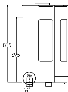
WESTFIRE.UNIQ.36 WESTFIRE.UNIQ.37 LEGS / WEIGHT: 85 KG
