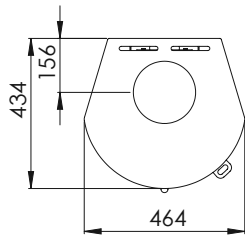
WESTFIRE.UNIQ.23 INSERT 4-SIDED FRAME FLAT / CURVED DOOR WEIGHT: 92 KG
