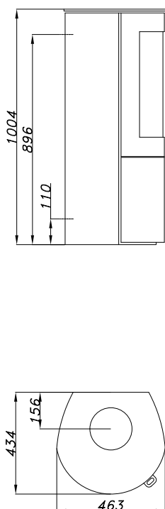
WESTFIRE.UNIQ.26 WEIGHT: 105 KG
